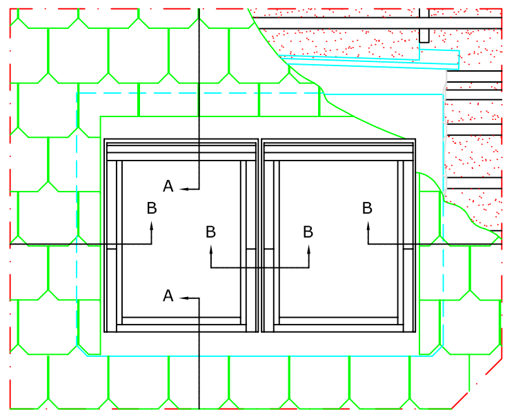
TYPICAL ELEVATION
