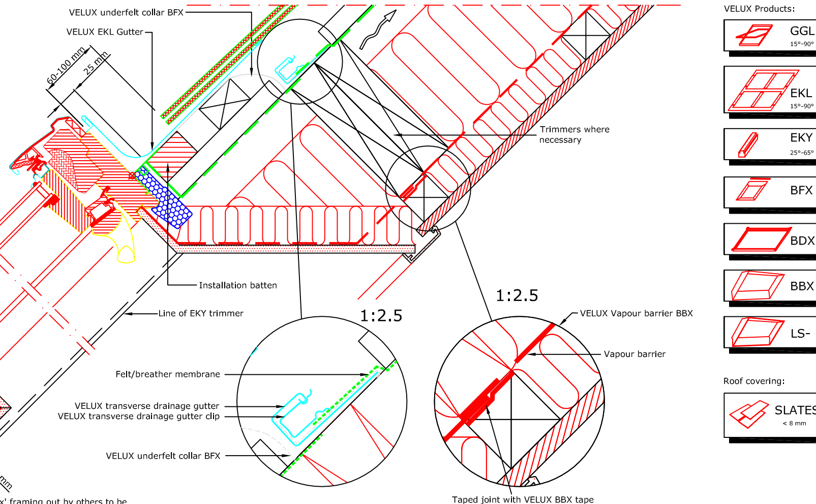
Section B-B 1:5
