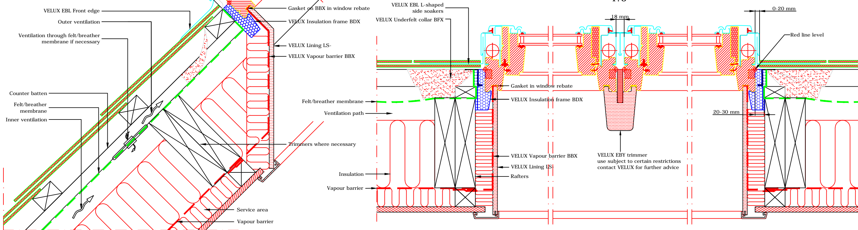
Section B-B 1:5
