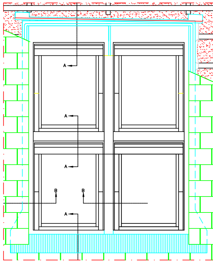
TYPICAL ELEVATION
